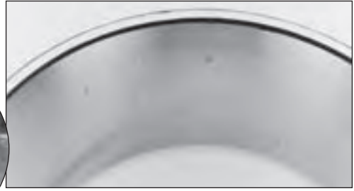
Roller spaced nicking Raised metal on races from contact with roller edges.
